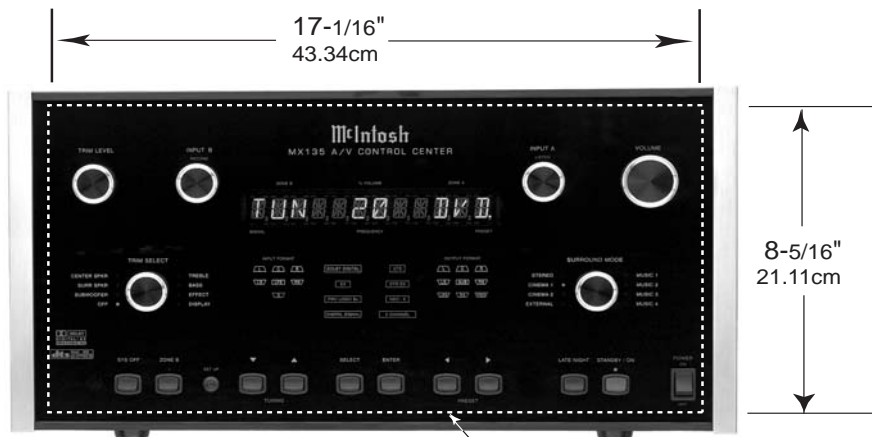
MX135 Front Panel Custom Cabinet Cutout
